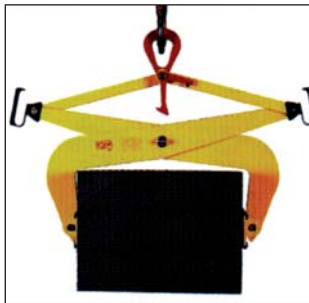
PB Clamp for lifting loads with parallel sides
