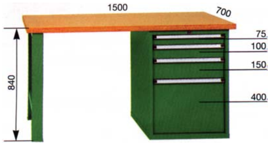
N-WSB 150/80 Work Bench
