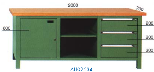
P-KW 200 Work Bench
